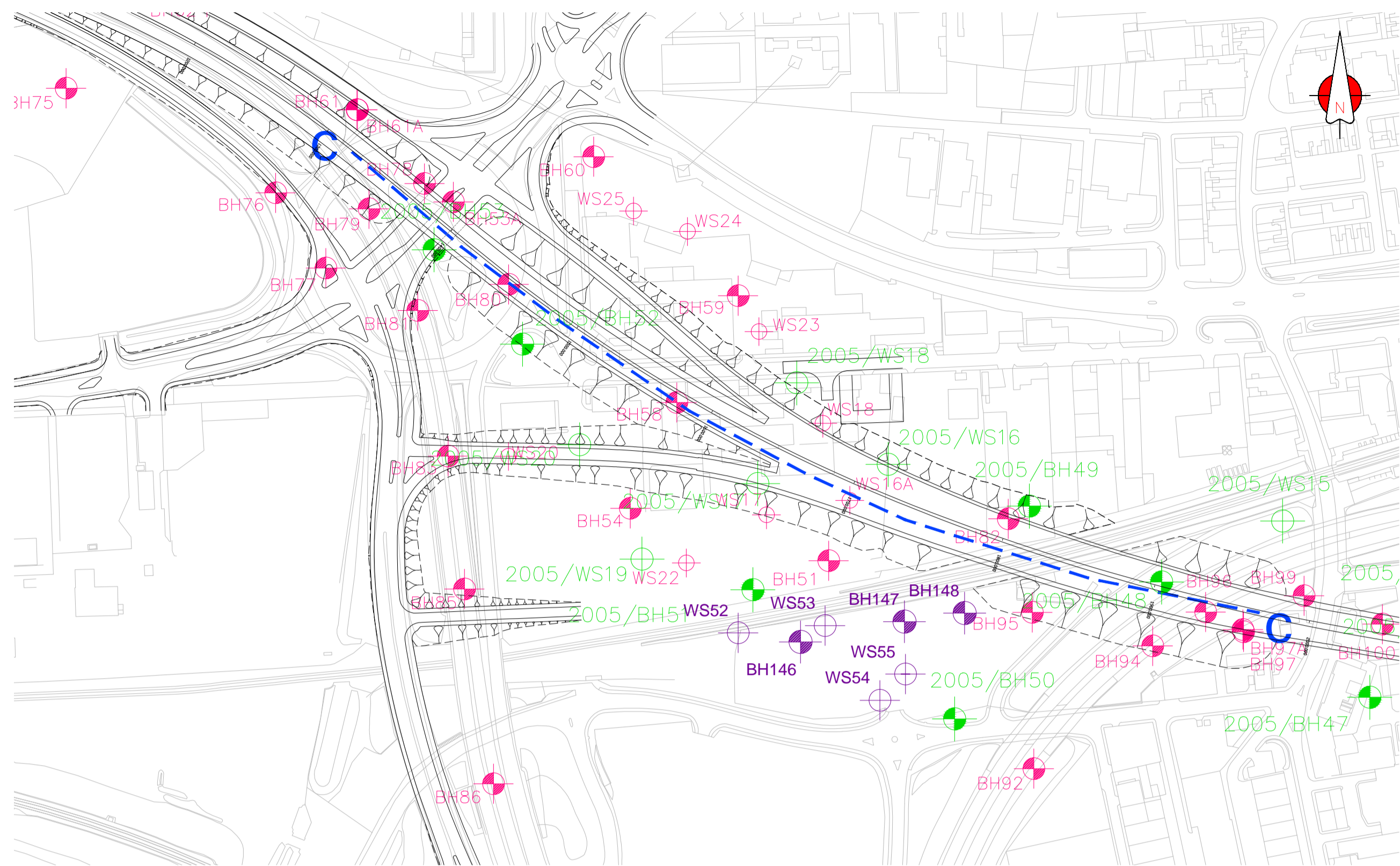
Plan view Section C-C 1:5000
