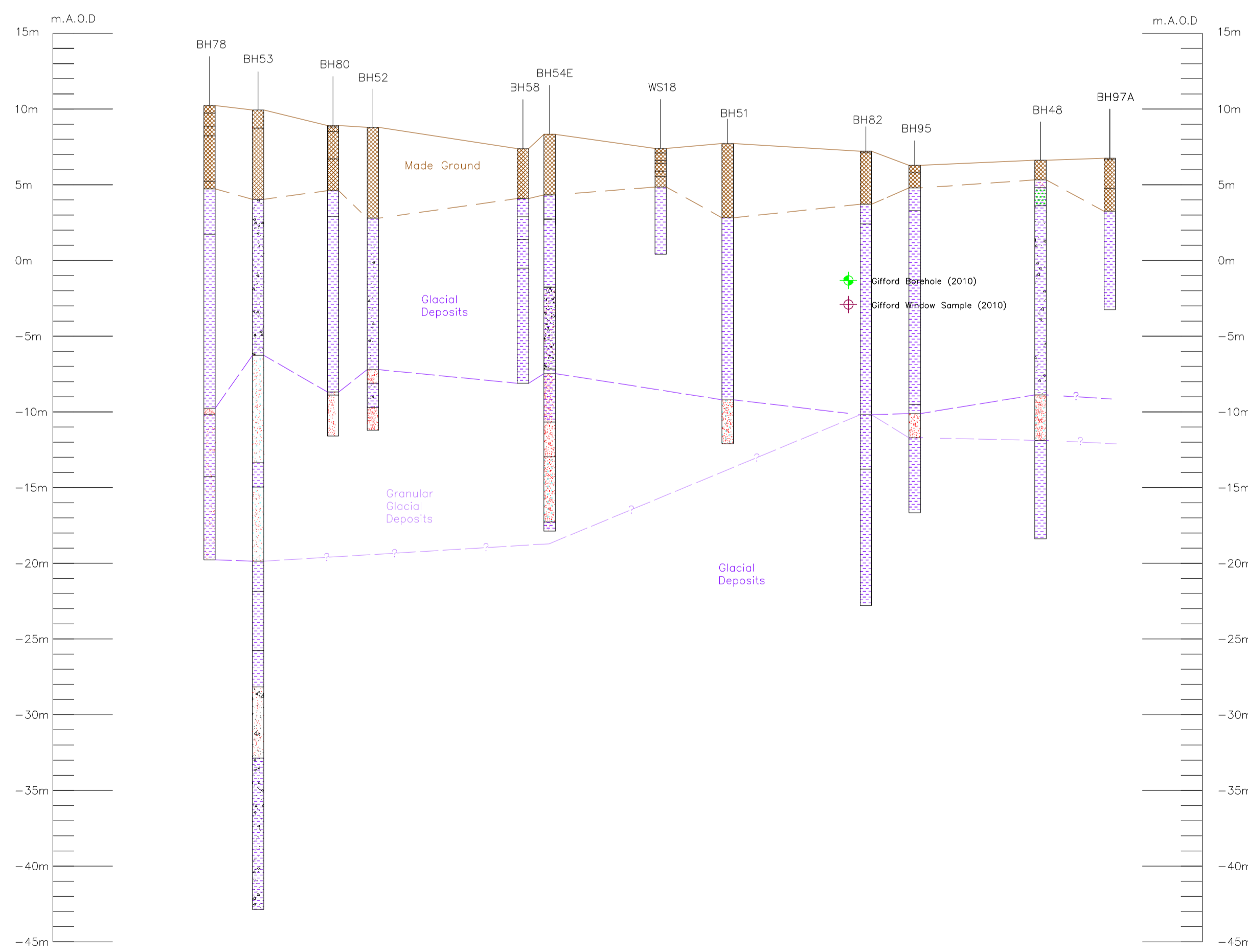
Section C-C Horizontal Scale 1:5000 Vertical Scale 1:500
